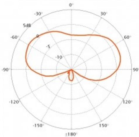
65000 Radiation pattern
